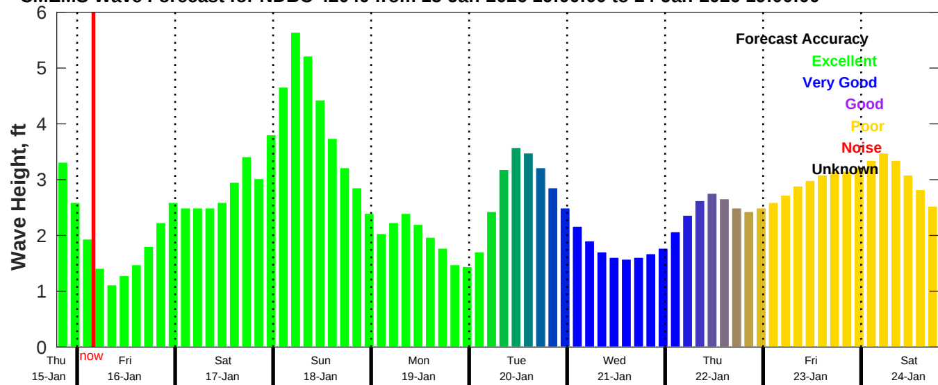
CMEMS Wave Forecast for NDBC 42040 from 15-Jan-2026 19:00:00 to 24-Jan-2026 19:00:00
