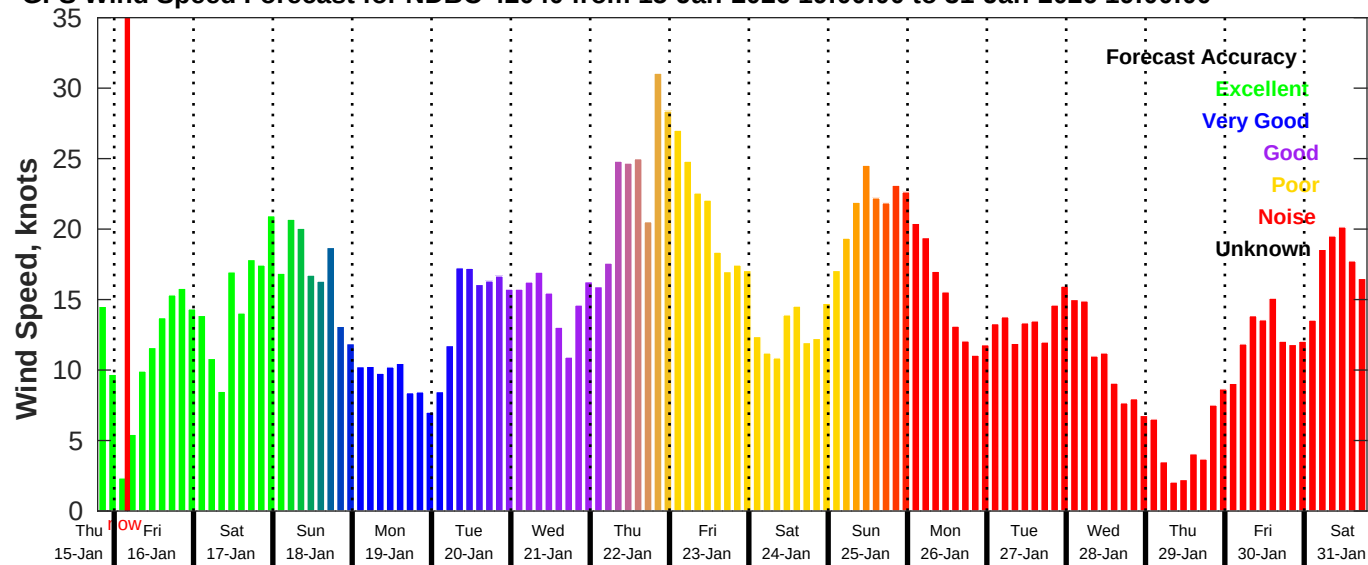
GFS Wind Speed Forecast for NDBC 42040 from 15-Jan-2026 19:00:00 to 31-Jan-2026 19:00:00
