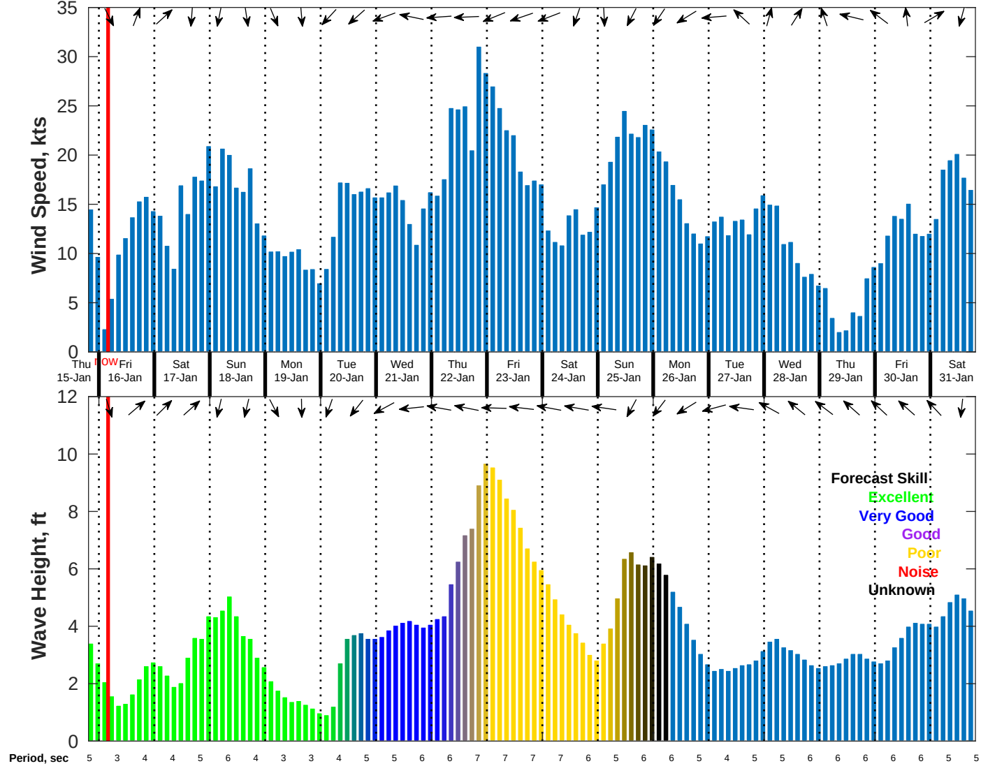
Wind & Wave Forecast for NDBC 42040 from 15-Jan-2026 19:00:00 to 31-Jan-2026 19:00:00
