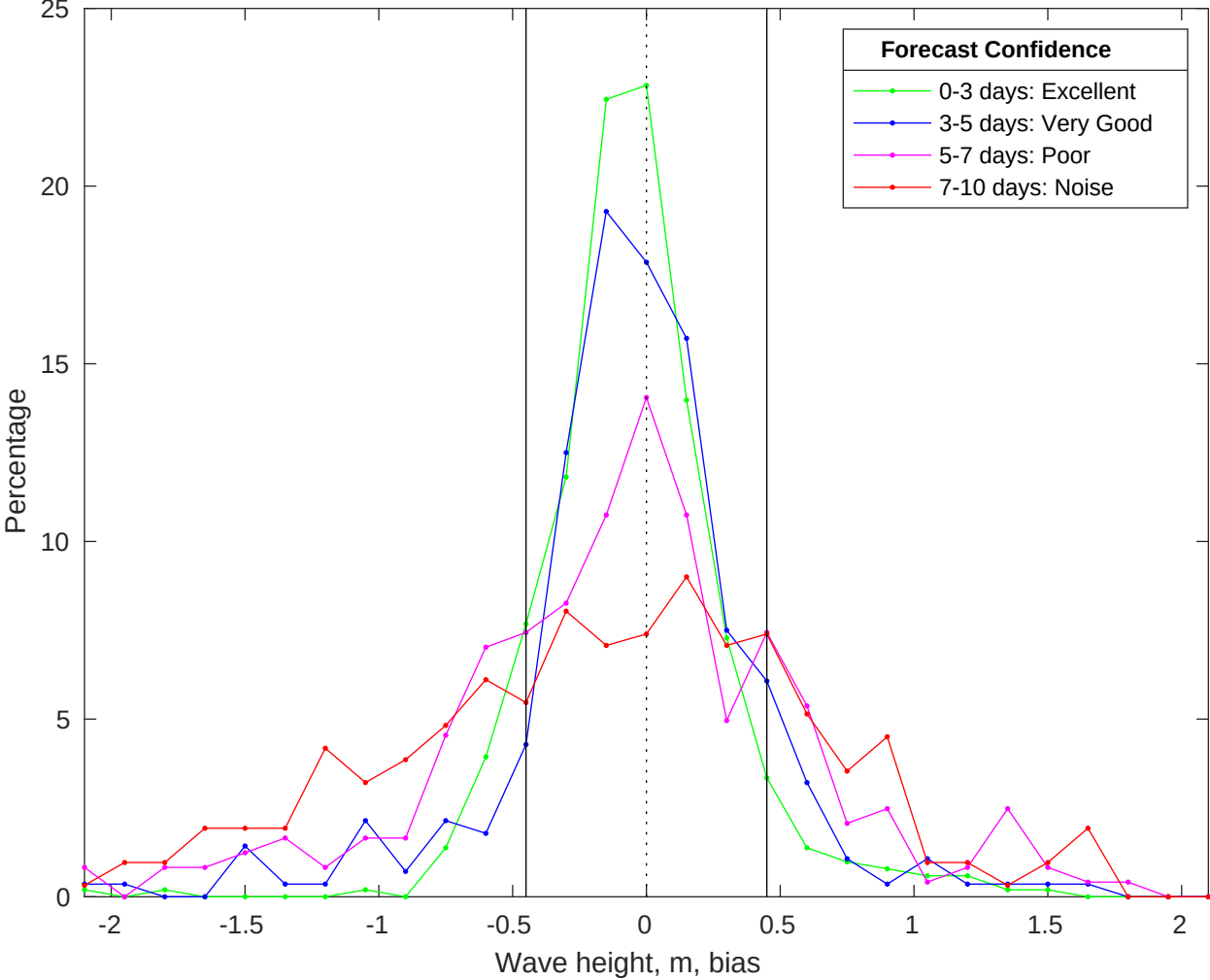
NDBC 44008 vs CMEMS Waves Bias Histogram: 16-Jan-2026
