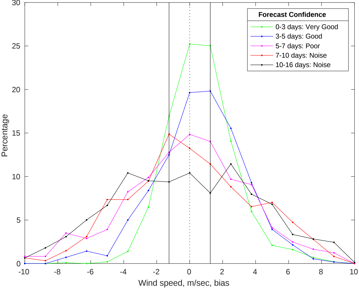
NDBC 44008 vs GFS Winds Bias Histogram: 16-Jan-2026
