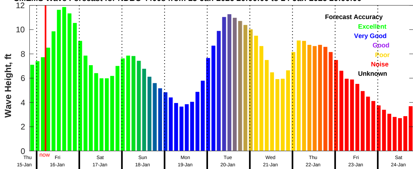
CMEMS Wave Forecast for NDBC 44008 from 15-Jan-2026 20:00:00 to 24-Jan-2026 20:00:00
