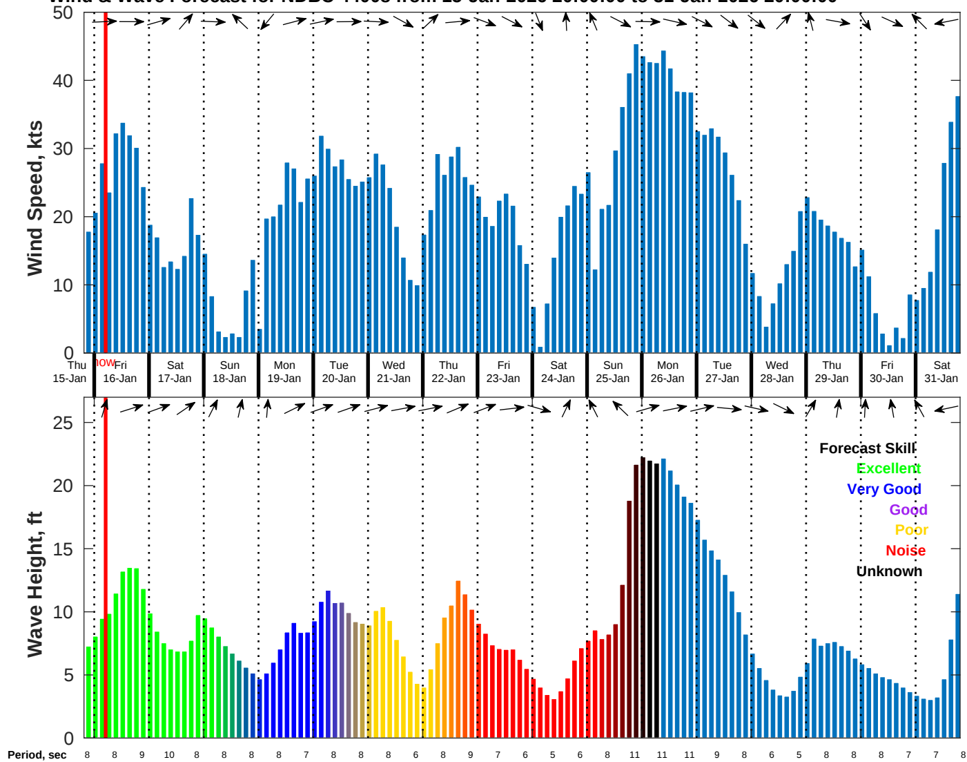
Wind & Wave Forecast for NDBC 44008 from 15-Jan-2026 20:00:00 to 31-Jan-2026 20:00:00
