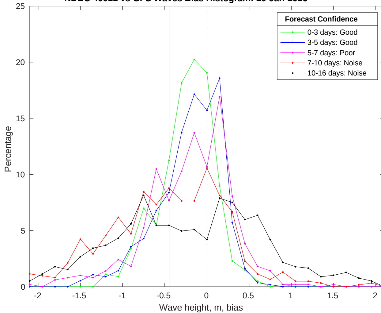
NDBC 46011 vs GFS Waves Bias Histogram: 16-Jan-2026
