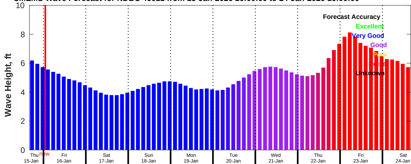
CMEMS Wave Forecast for NDBC 46011 from 15-Jan-2026 16:00:00 to 24-Jan-2026 16:00:00
