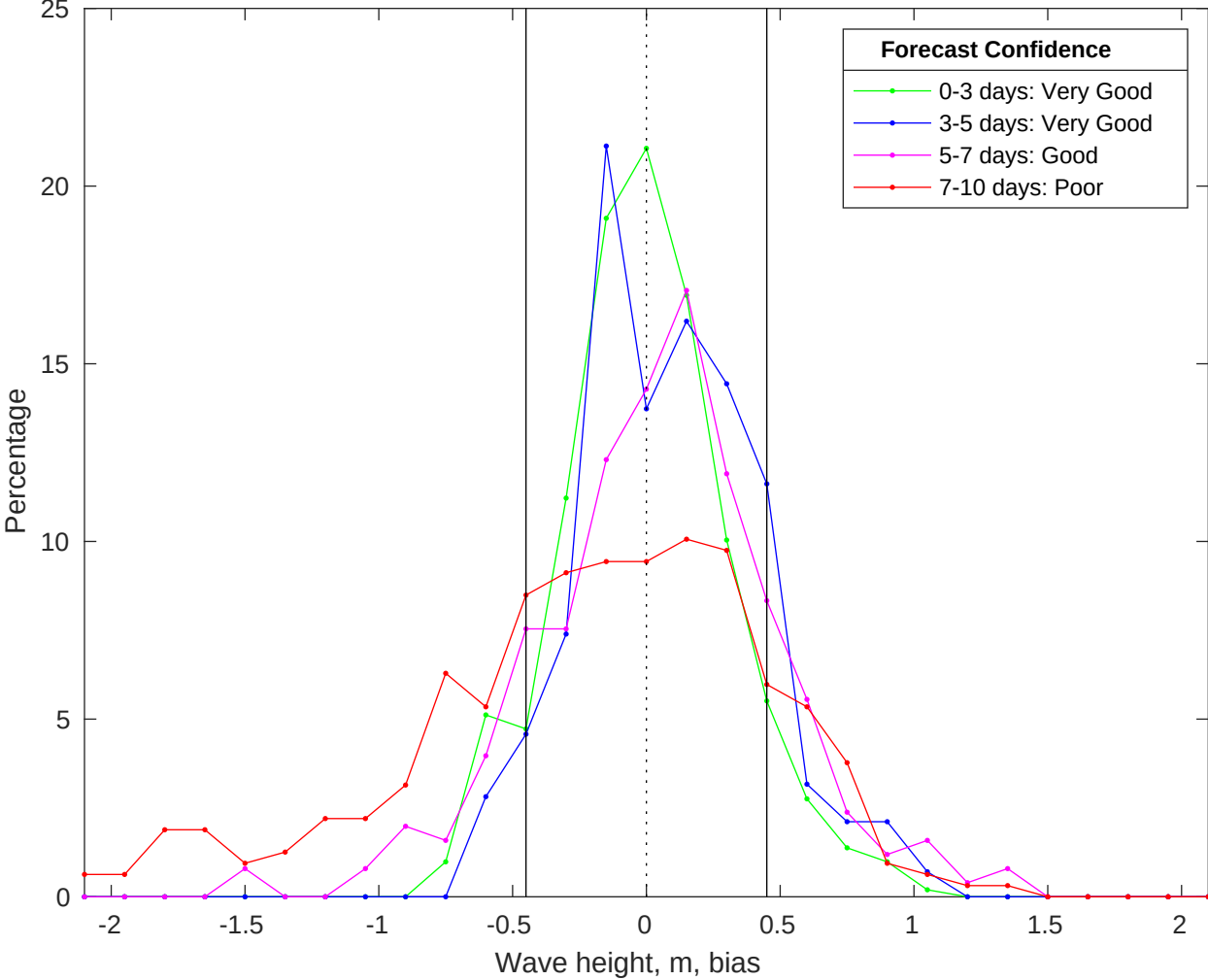
NDBC 46028 vs CMEMS Waves Bias Histogram: 16-Jan-2026
