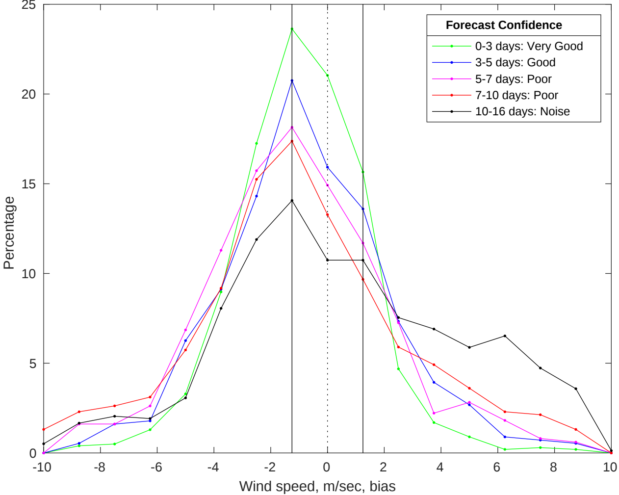
NDBC 46028 vs GFS Winds Bias Histogram: 16-Jan-2026
