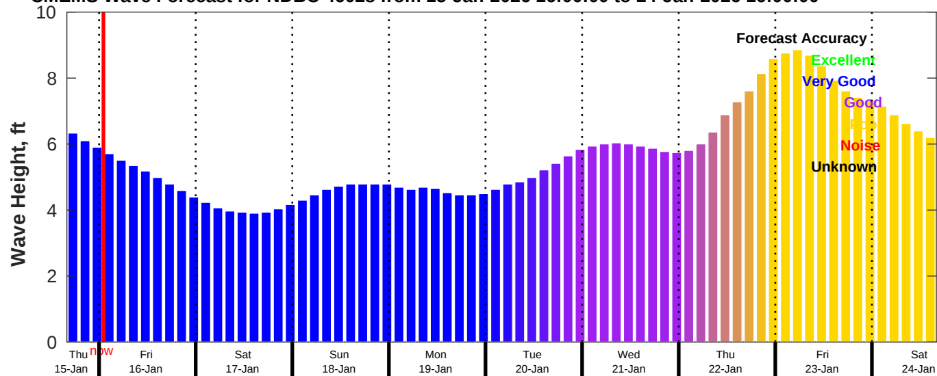
CMEMS Wave Forecast for NDBC 46028 from 15-Jan-2026 16:00:00 to 24-Jan-2026 16:00:00
