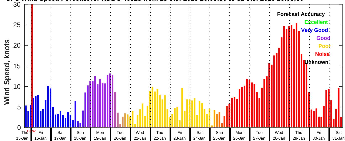
GFS Wind Speed Forecast for NDBC 46028 from 15-Jan-2026 16:00:00 to 31-Jan-2026 16:00:00
