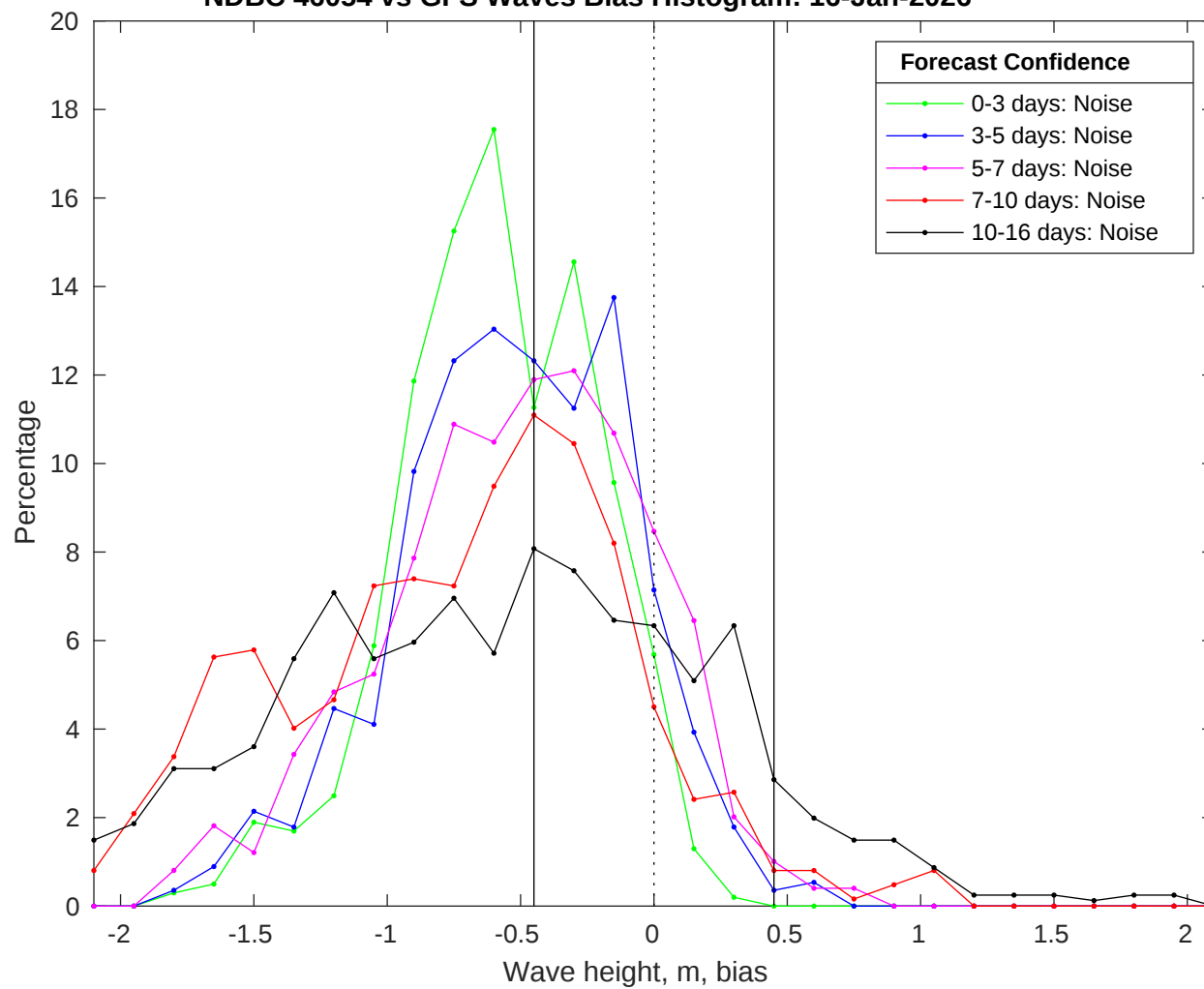
NDBC 46054 vs GFS Waves Bias Histogram: 16-Jan-2026
