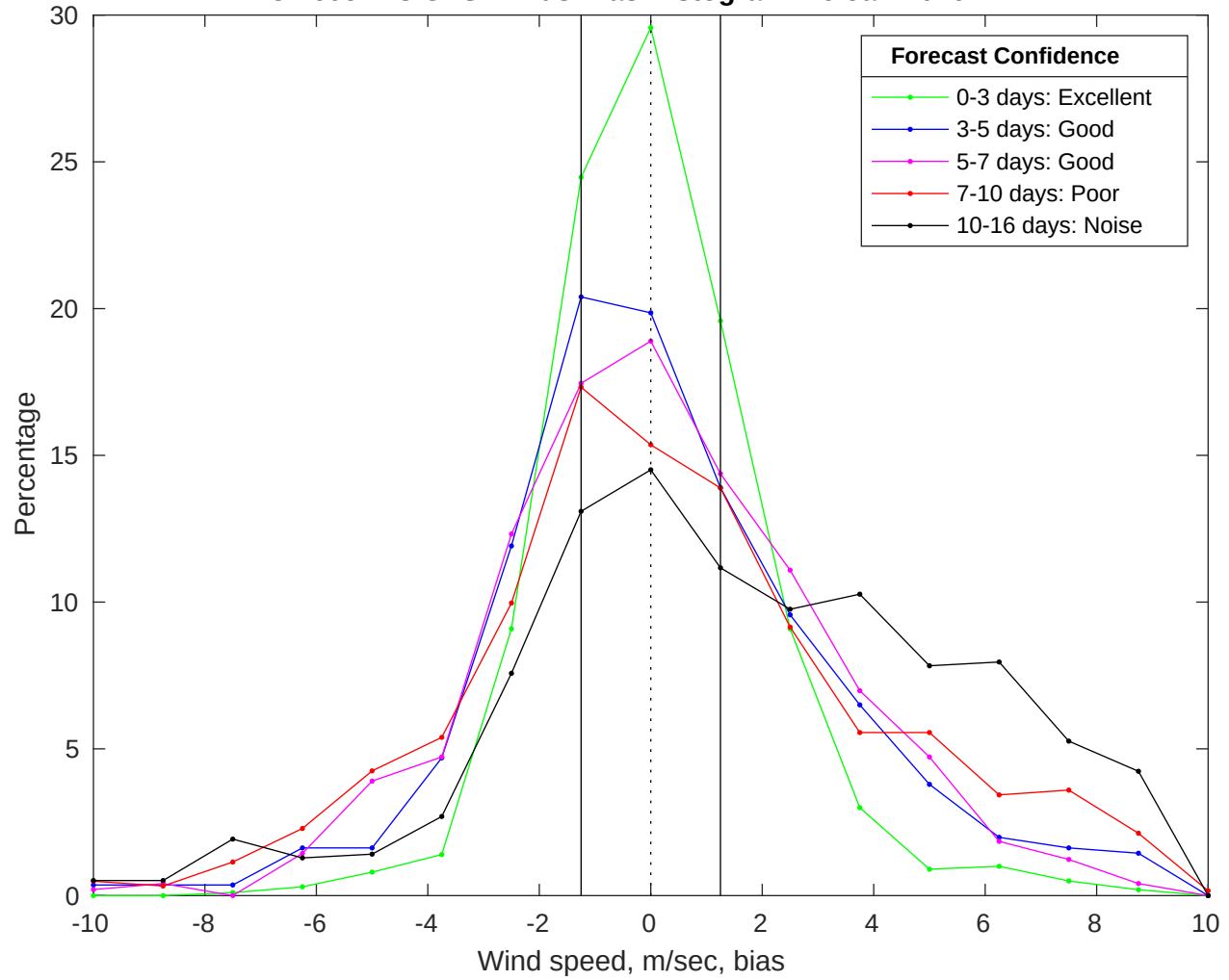
NDBC 46054 vs GFS Winds Bias Histogram: 16-Jan-2026
