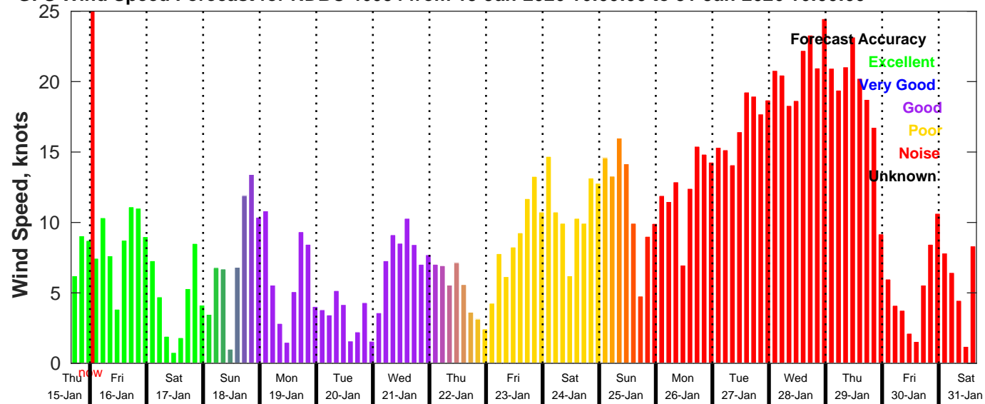
GFS Wind Speed Forecast for NDBC 46054 from 15-Jan-2026 16:00:00 to 31-Jan-2026 16:00:00
