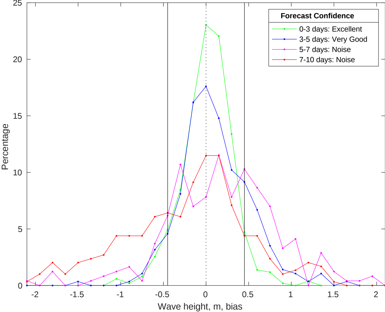
NDBC 46059 vs CMEMS Waves Bias Histogram: 16-Jan-2026
