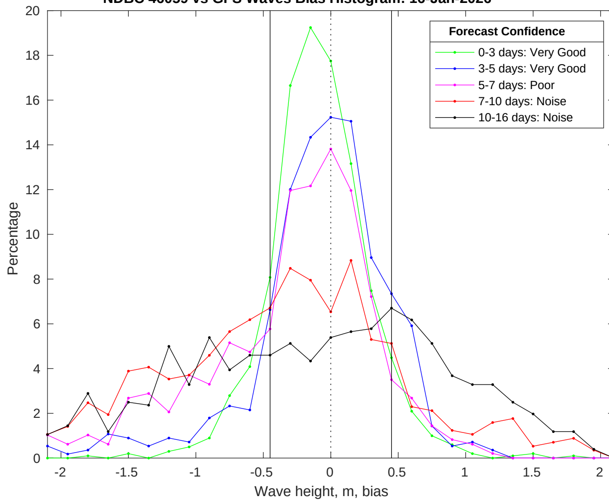
NDBC 46059 vs GFS Waves Bias Histogram: 16-Jan-2026
