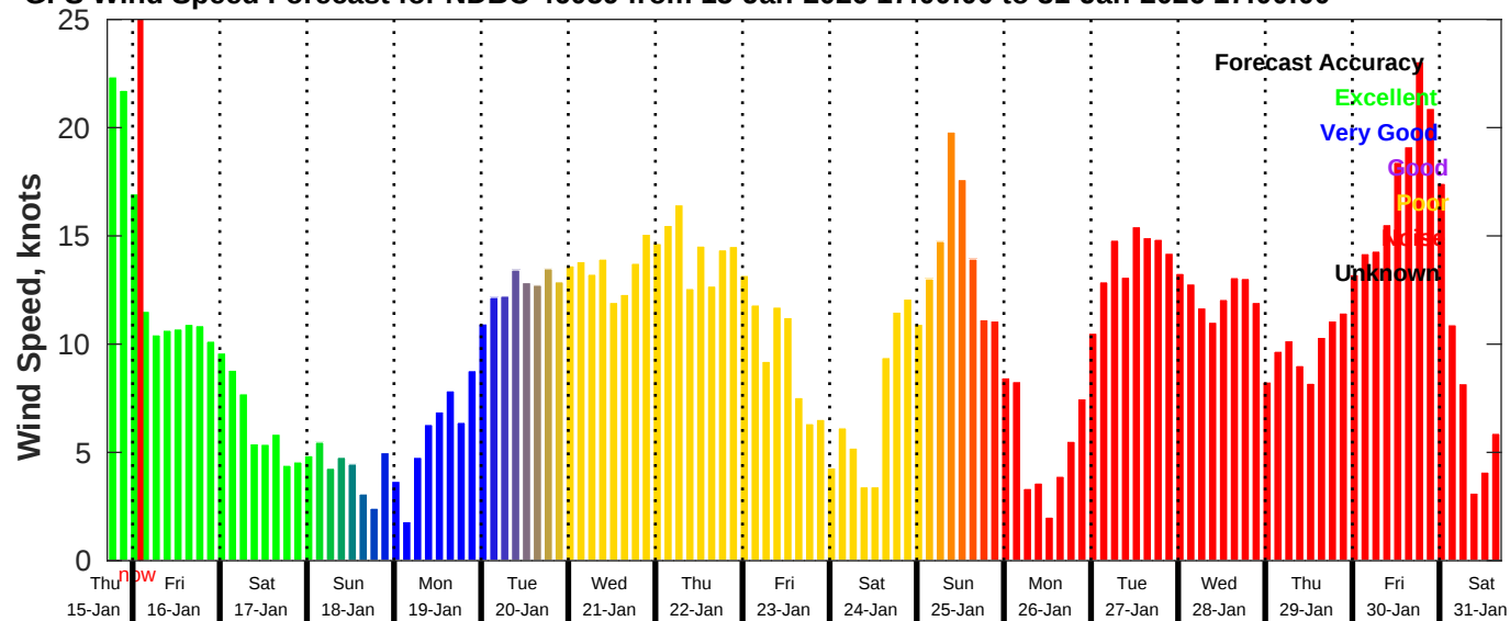
GFS Wind Speed Forecast for NDBC 46059 from 15-Jan-2026 17:00:00 to 31-Jan-2026 17:00:00
