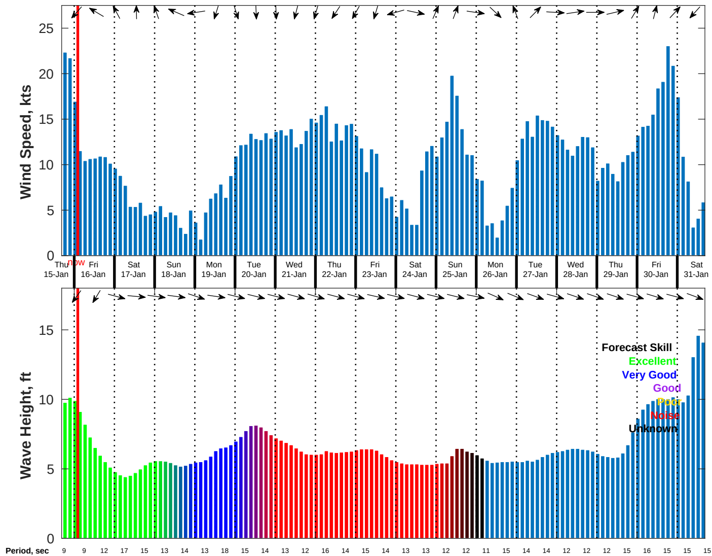
Wind & Wave Forecast for NDBC 46059 from 15-Jan-2026 17:00:00 to 31-Jan-2026 17:00:00
