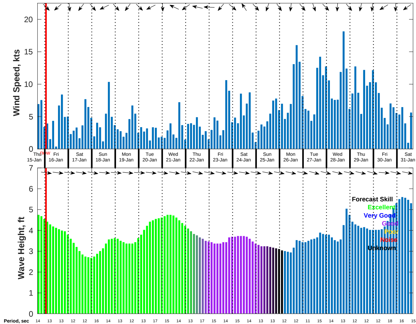
Wind & Wave Forecast for NDBC 46215 from 15-Jan-2026 16:00:00 to 31-Jan-2026 16:00:00
