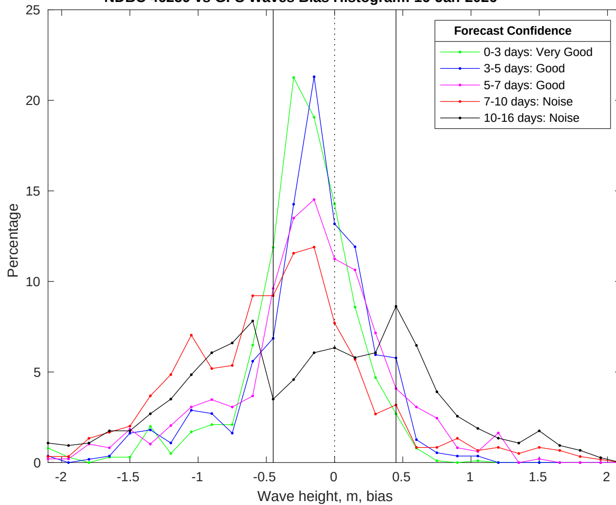
NDBC 46259 vs GFS Waves Bias Histogram: 16-Jan-2026
