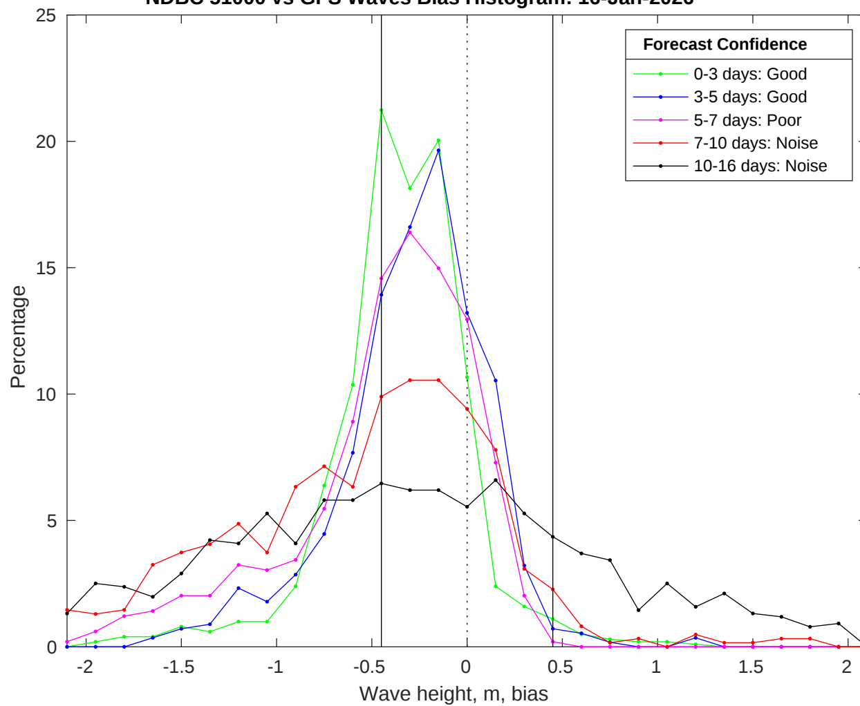
NDBC 51000 vs GFS Waves Bias Histogram: 16-Jan-2026
