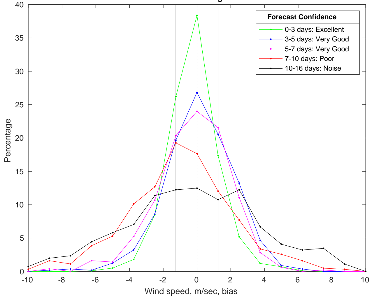
NDBC 51000 vs GFS Winds Bias Histogram: 16-Jan-2026
