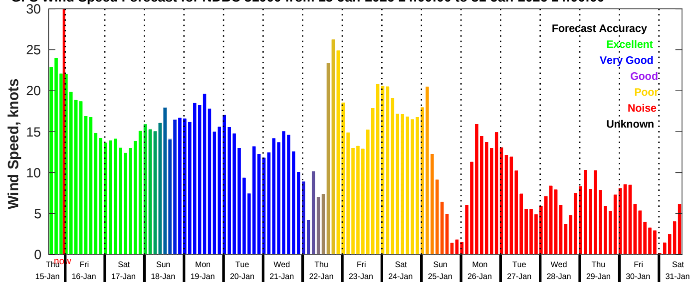
GFS Wind Speed Forecast for NDBC 51000 from 15-Jan-2026 14:00:00 to 31-Jan-2026 14:00:00
