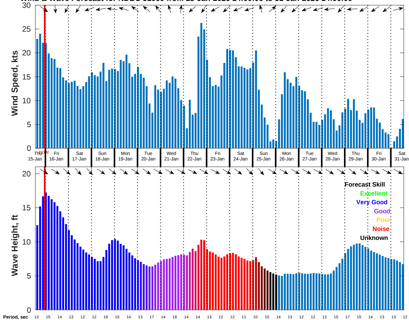
Wind & Wave Forecast for NDBC 51000 from 15-Jan-2026 14:00:00 to 31-Jan-2026 14:00:00
