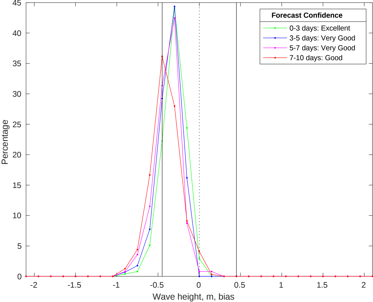
NDBC 51209 vs CMEMS Waves Bias Histogram: 16-Jan-2026
