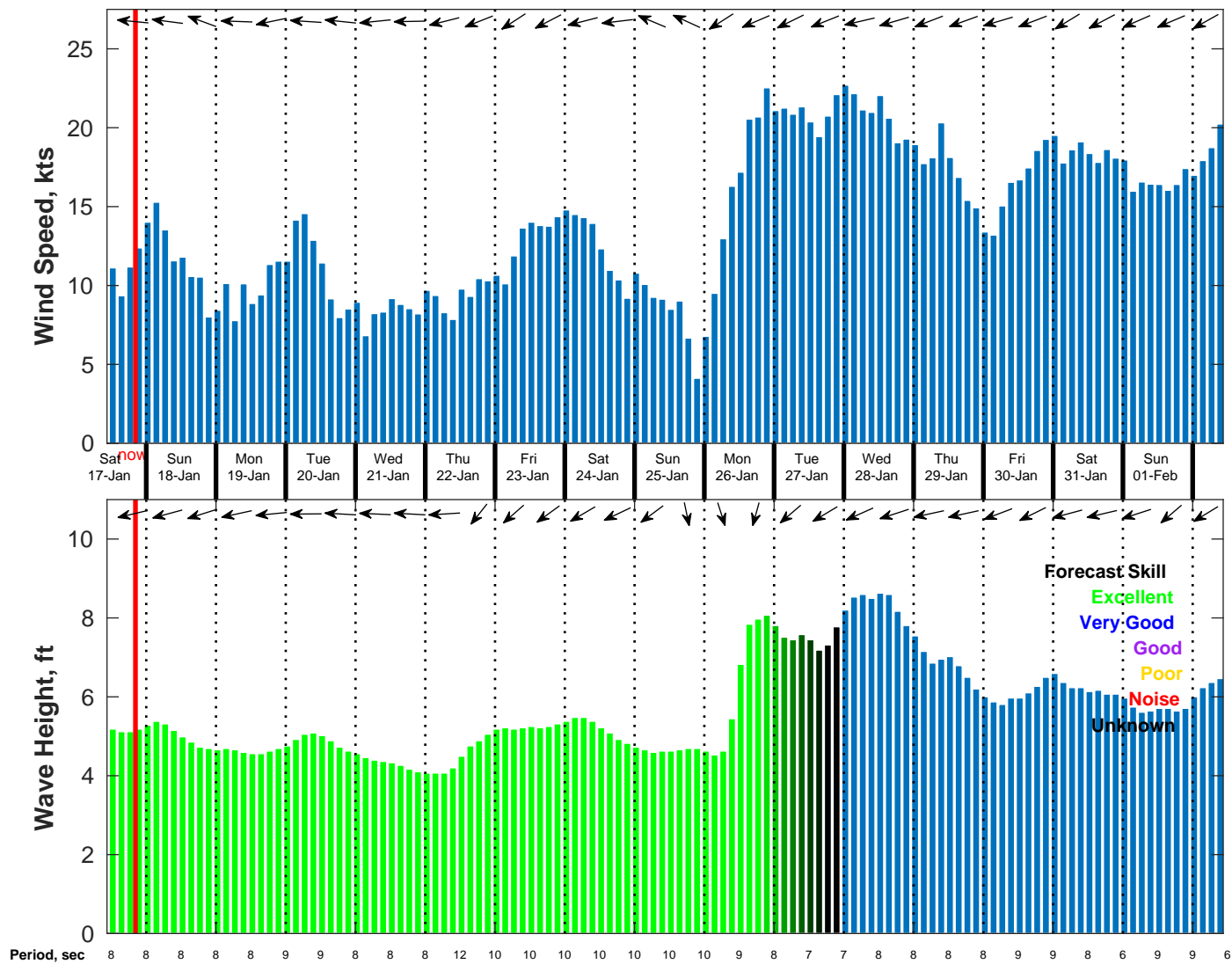
Wind & Wave Forecast for NDBC 52211 from 16-Jan-2026 11:00:00 to 01-Feb-2026 11:00:00
