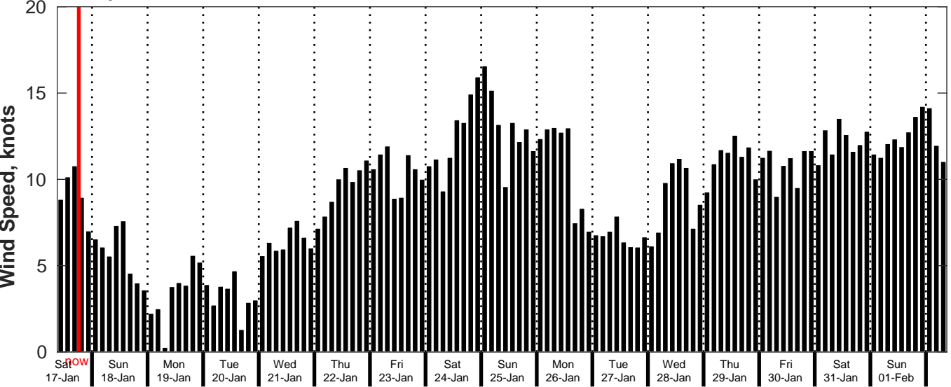
GFS Wind Speed Forecast for NDBC 52212 from 16-Jan-2026 09:00:00 to 01-Feb-2026 09:00:00
