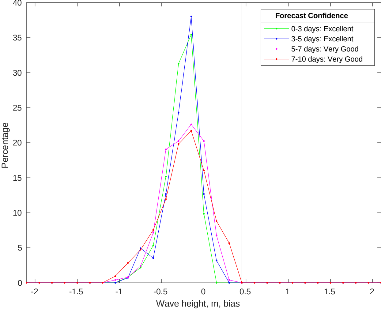
NDBC 52213 vs CMEMS Waves Bias Histogram: 16-Jan-2026
