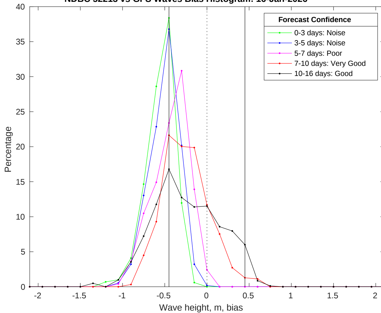
NDBC 52213 vs GFS Waves Bias Histogram: 16-Jan-2026
