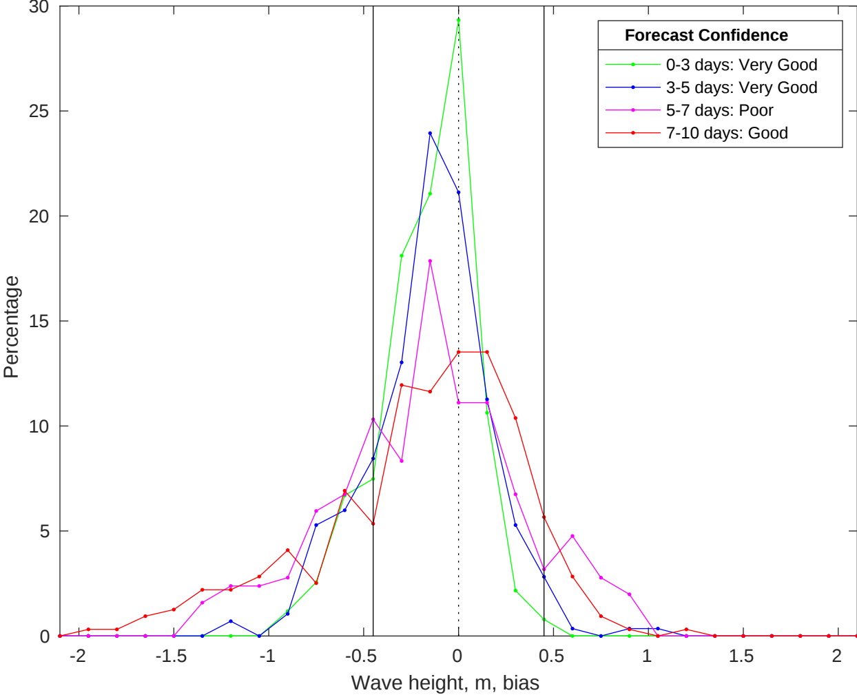
NDBC 41004 vs CMEMS Waves Bias Histogram: 17-Jan-2026
