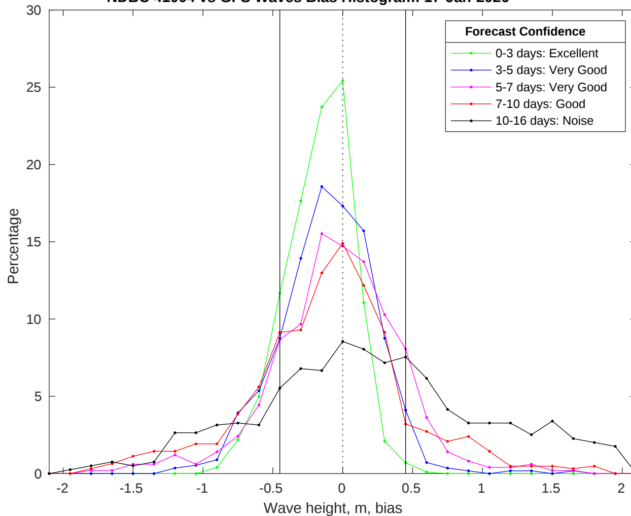
NDBC 41004 vs GFS Waves Bias Histogram: 17-Jan-2026
