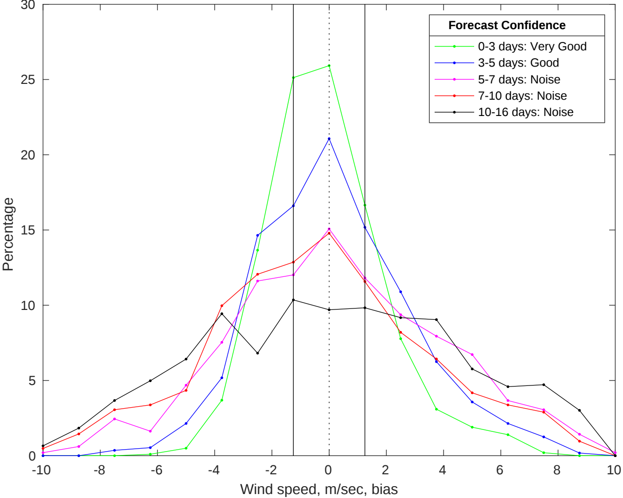
NDBC 41004 vs GFS Winds Bias Histogram: 17-Jan-2026
