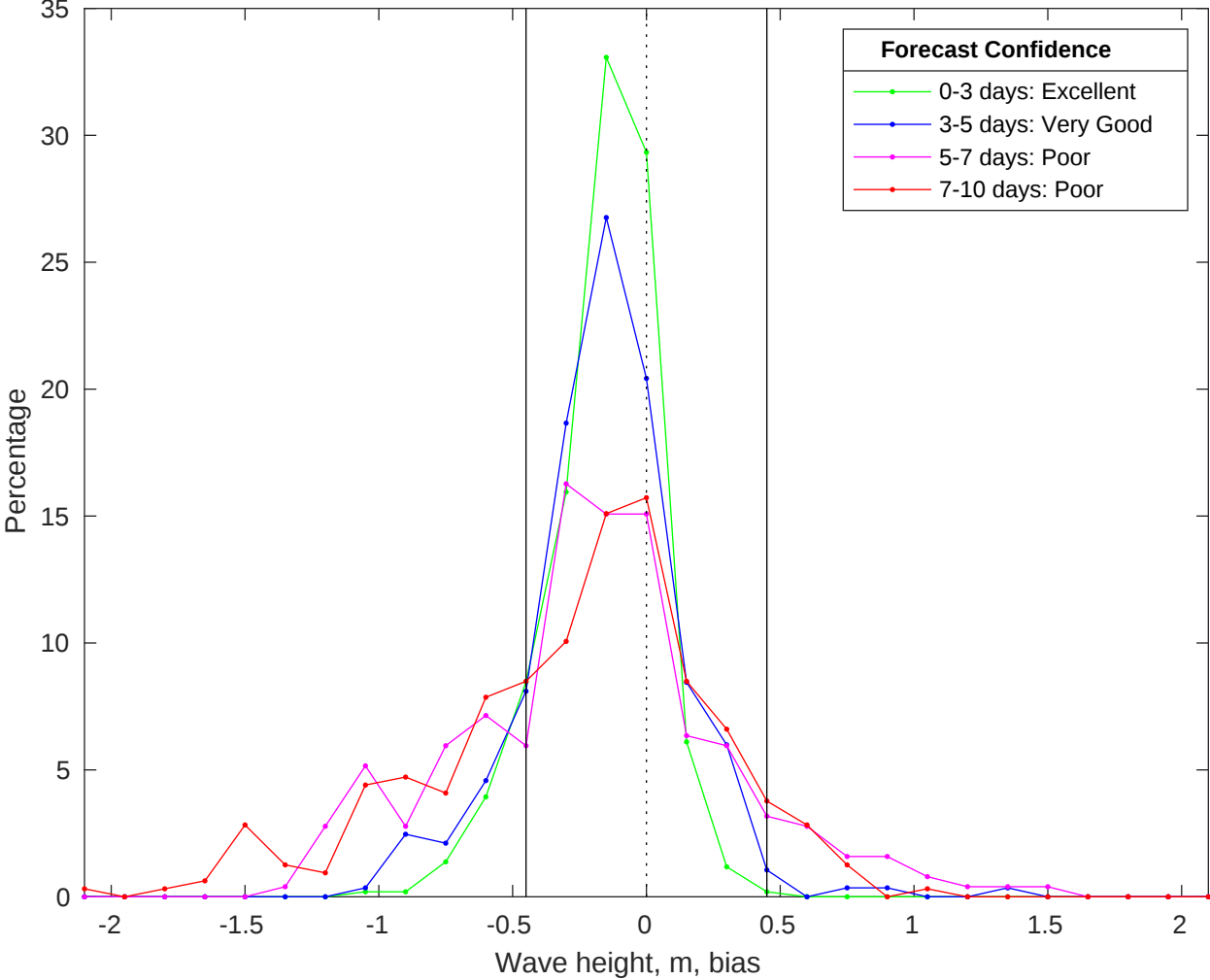
NDBC 41013 vs CMEMS Waves Bias Histogram: 17-Jan-2026
