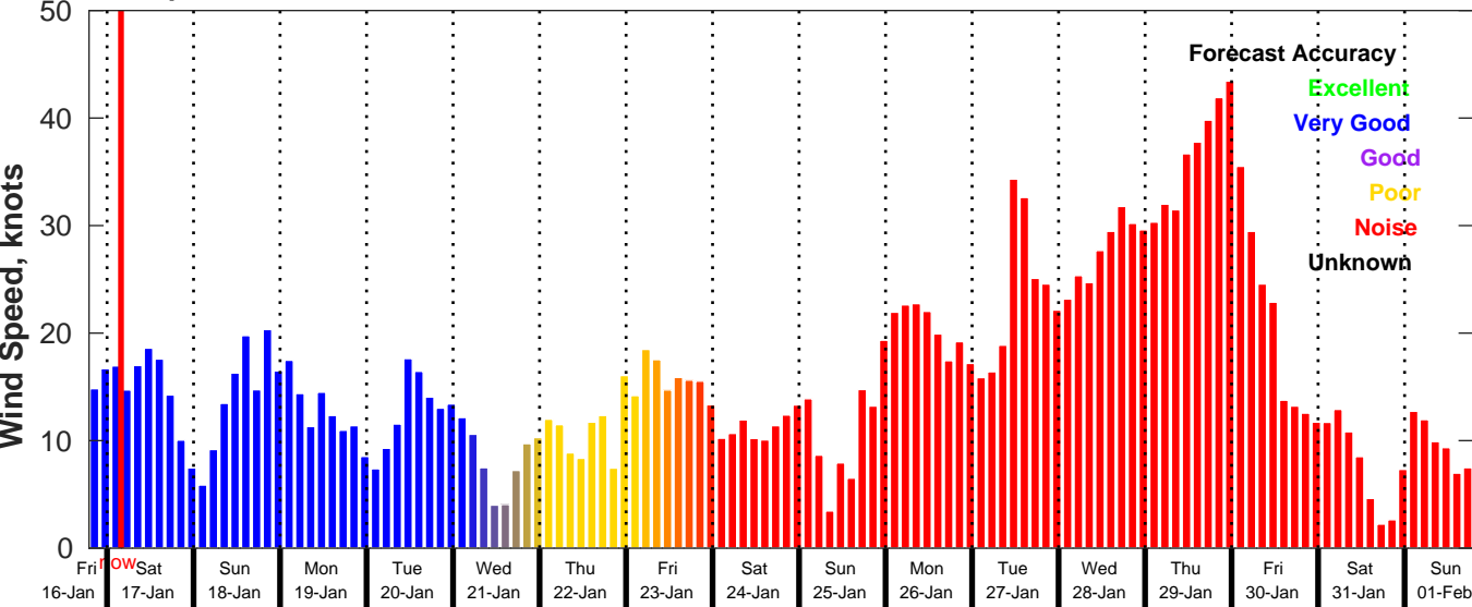
GFS Wind Speed Forecast for NDBC 41013 from 16-Jan-2026 19:00:00 to 01-Feb-2026 19:00:00
