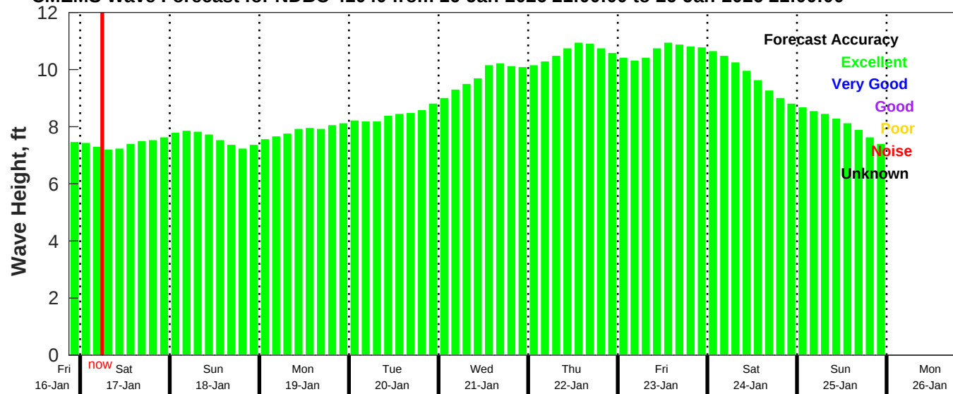
CMEMS Wave Forecast for NDBC 41040 from 16-Jan-2026 21:00:00 to 26-Jan-2026 21:00:00
