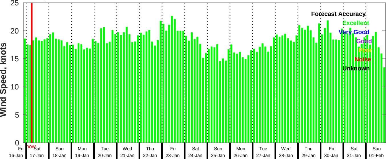
GFS Wind Speed Forecast for NDBC 41040 from 16-Jan-2026 21:00:00 to 01-Feb-2026 21:00:00
