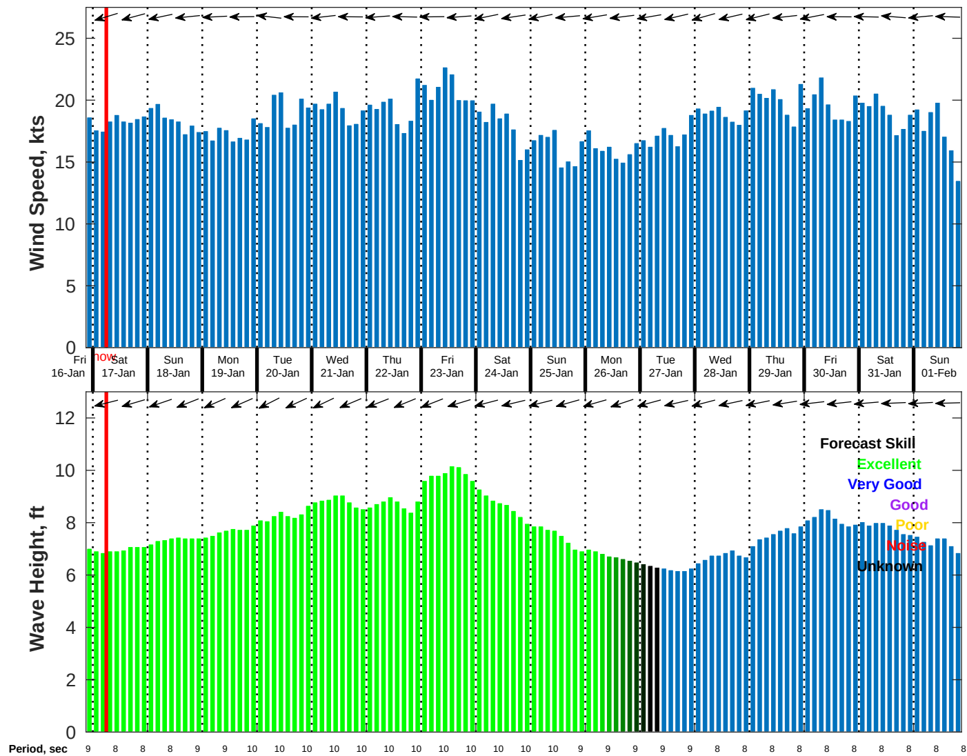
Wind & Wave Forecast for NDBC 41040 from 16-Jan-2026 21:00:00 to 01-Feb-2026 21:00:00
