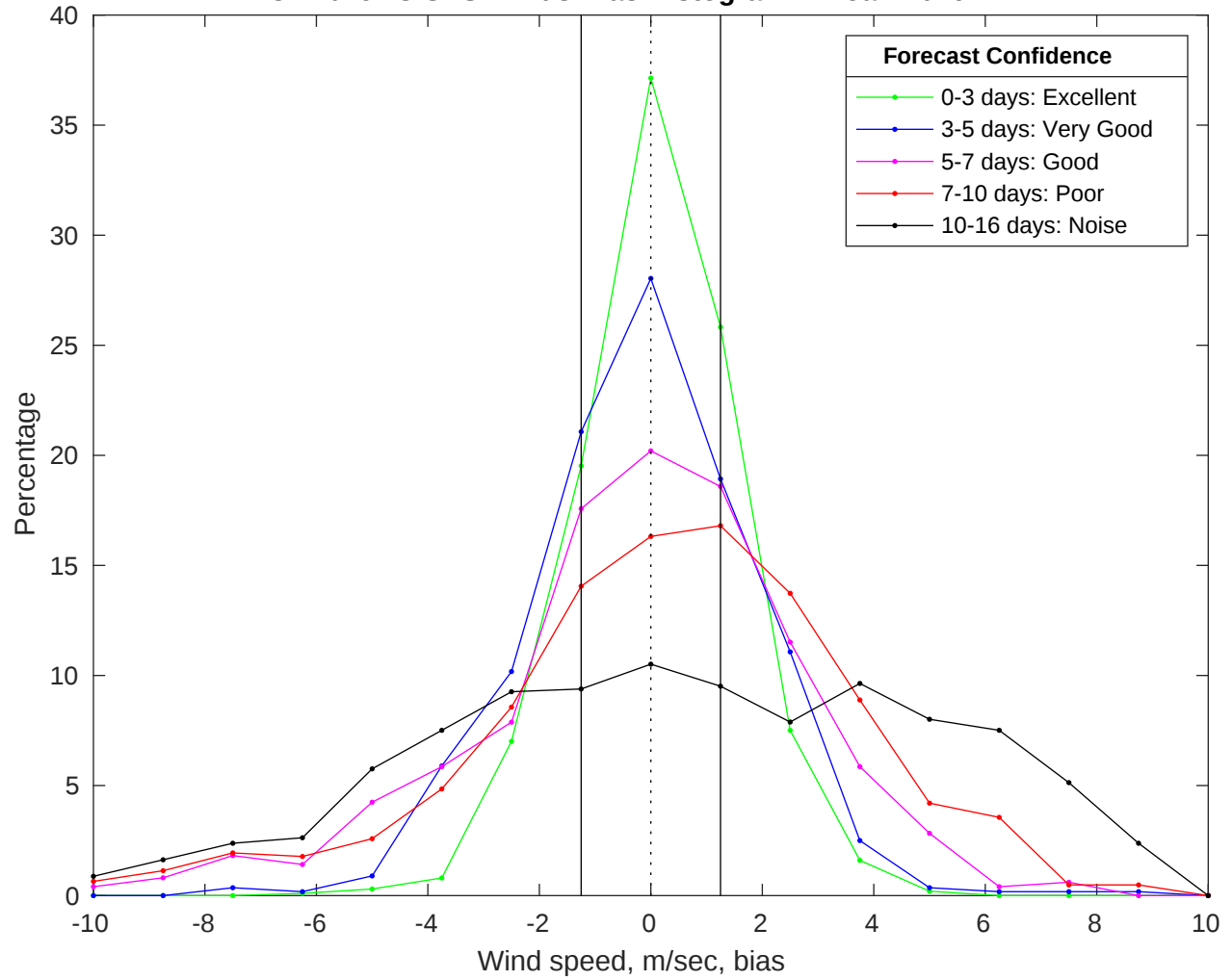
NDBC 42019 vs GFS Winds Bias Histogram: 17-Jan-2026
