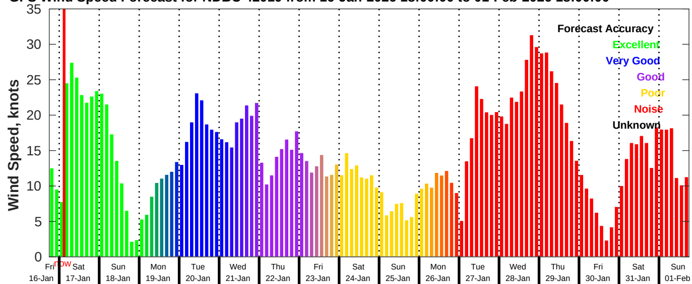
GFS Wind Speed Forecast for NDBC 42019 from 16-Jan-2026 18:00:00 to 01-Feb-2026 18:00:00
