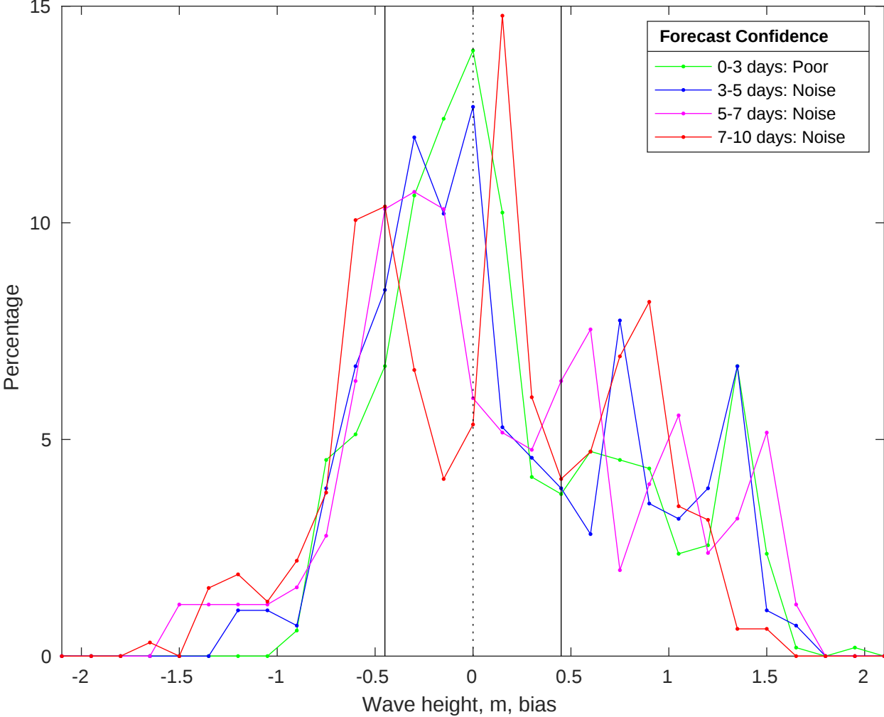
NDBC 42020 vs CMEMS Waves Bias Histogram: 17-Jan-2026
