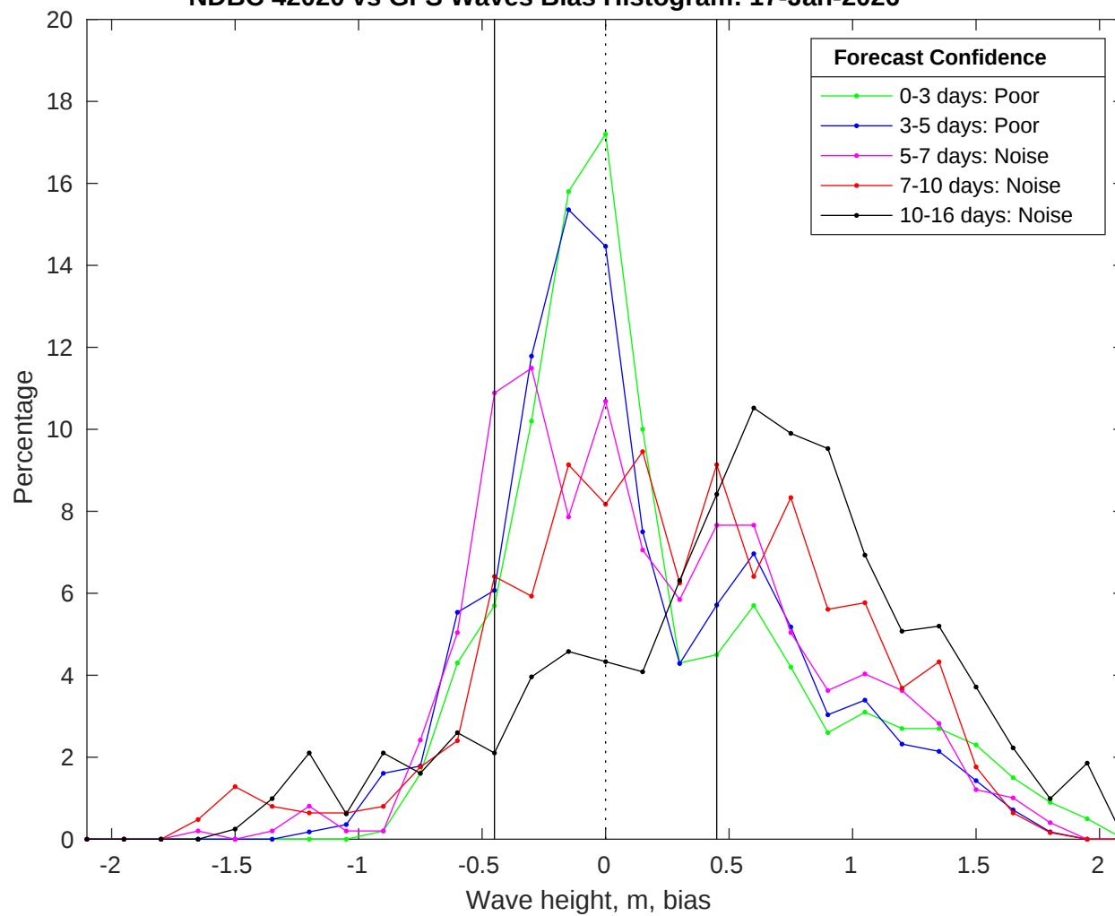
NDBC 42020 vs GFS Waves Bias Histogram: 17-Jan-2026
