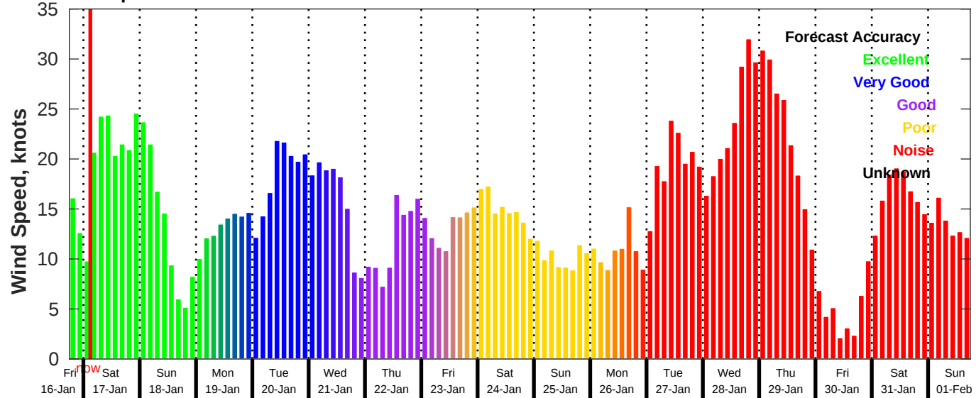
GFS Wind Speed Forecast for NDBC 42020 from 16-Jan-2026 18:00:00 to 01-Feb-2026 18:00:00
