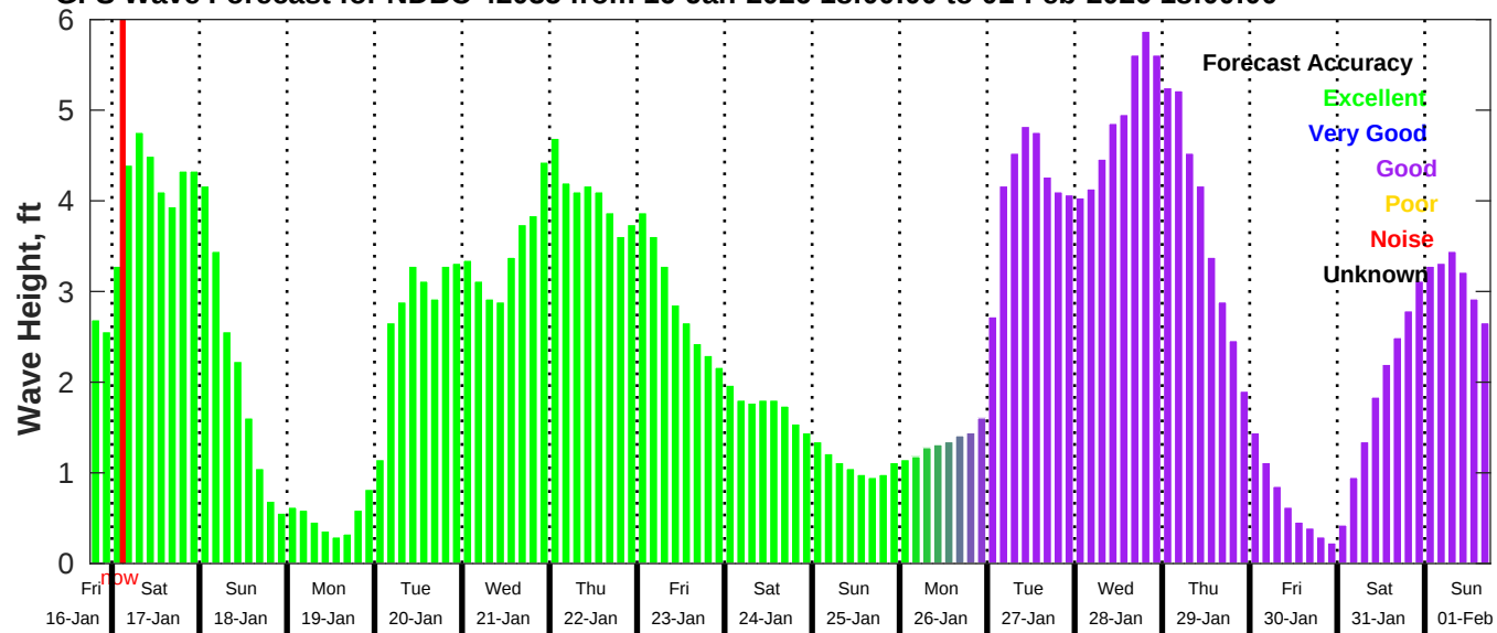
GFS Wave Forecast for NDBC 42035 from 16-Jan-2026 18:00:00 to 01-Feb-2026 18:00:00
