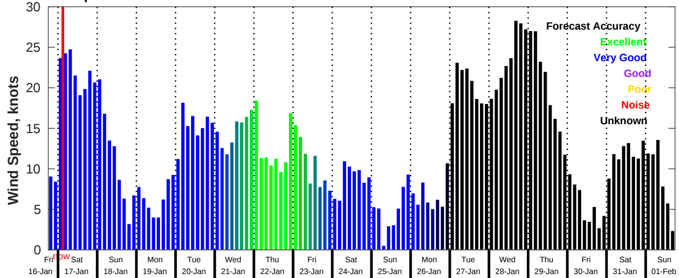
GFS Wind Speed Forecast for NDBC 42035 from 16-Jan-2026 18:00:00 to 01-Feb-2026 18:00:00
