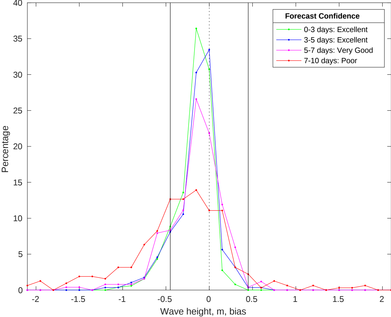
NDBC 42036 vs CMEMS Waves Bias Histogram: 17-Jan-2026
