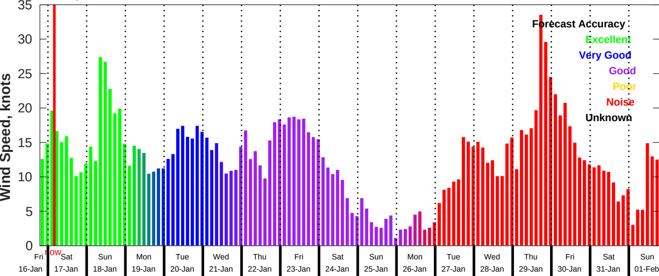
GFS Wind Speed Forecast for NDBC 42036 from 16-Jan-2026 19:00:00 to 01-Feb-2026 19:00:00
