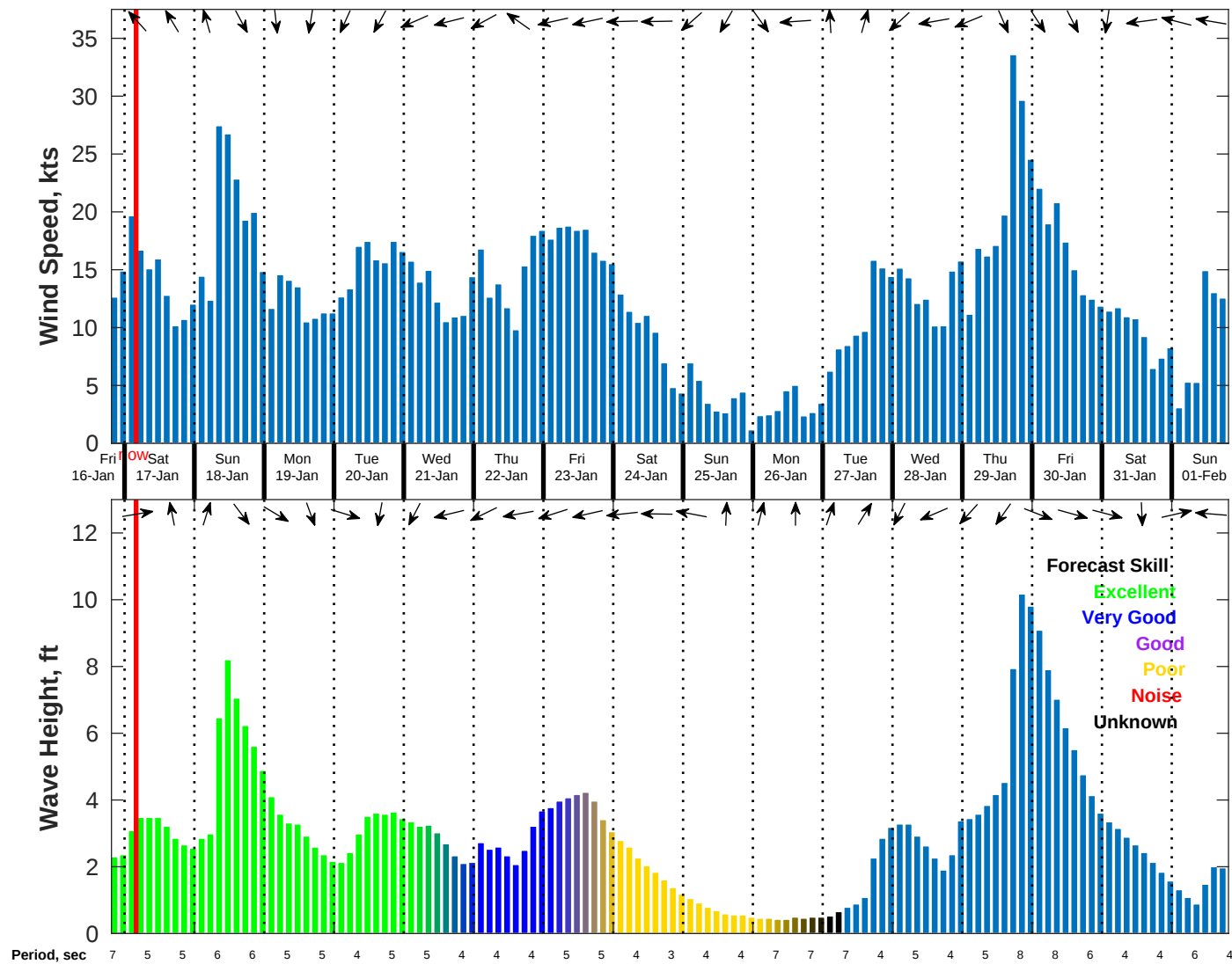
Wind & Wave Forecast for NDBC 42036 from 16-Jan-2026 19:00:00 to 01-Feb-2026 19:00:00
