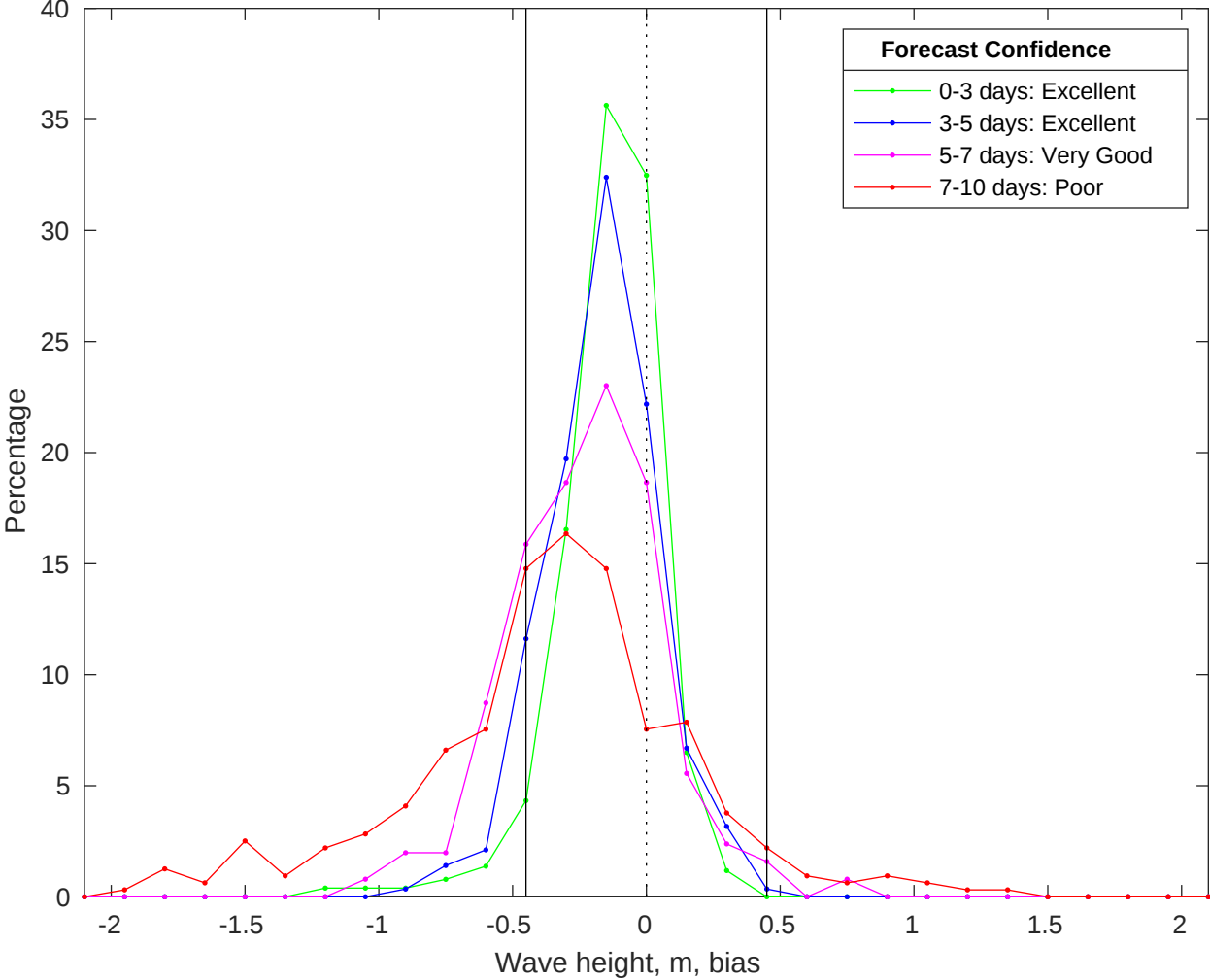
NDBC 42040 vs CMEMS Waves Bias Histogram: 17-Jan-2026
